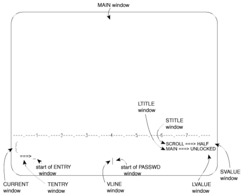
Figure 12. Session Manager Display Screen
